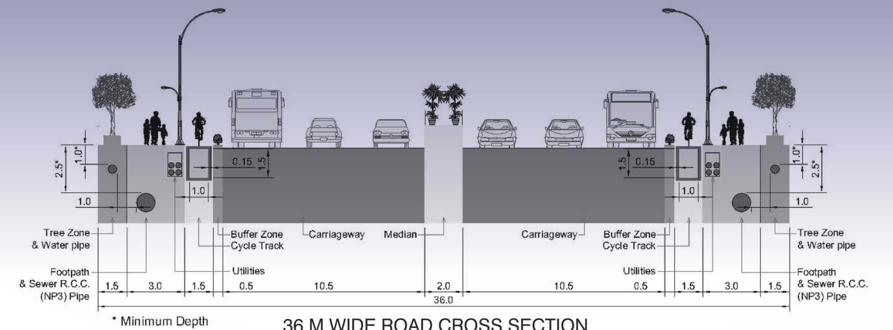
36 M WIDE ROAD CROSS SECTION
